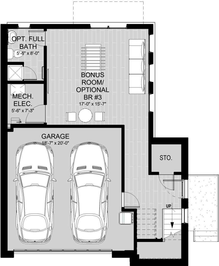
ENTRY LEVEL FLOOR PLAN
