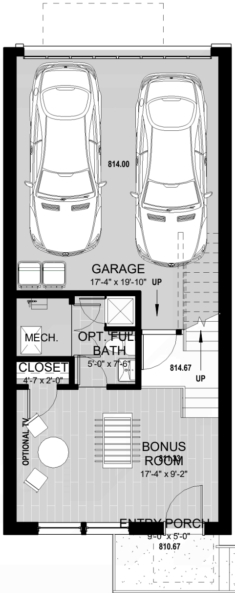
ENTRY LEVEL FLOOR PLAN
